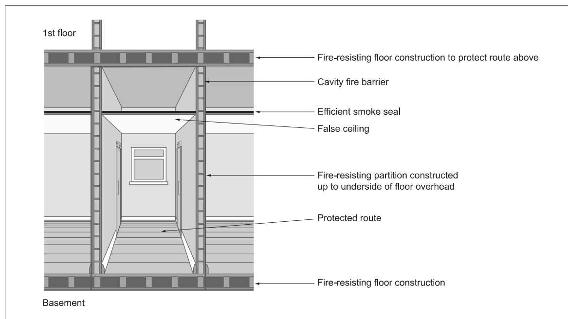
Figure 60: Fire-resisting construction
