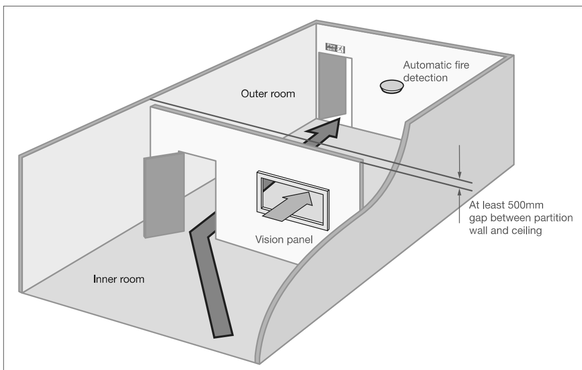
Figure 22: Inner rooms
